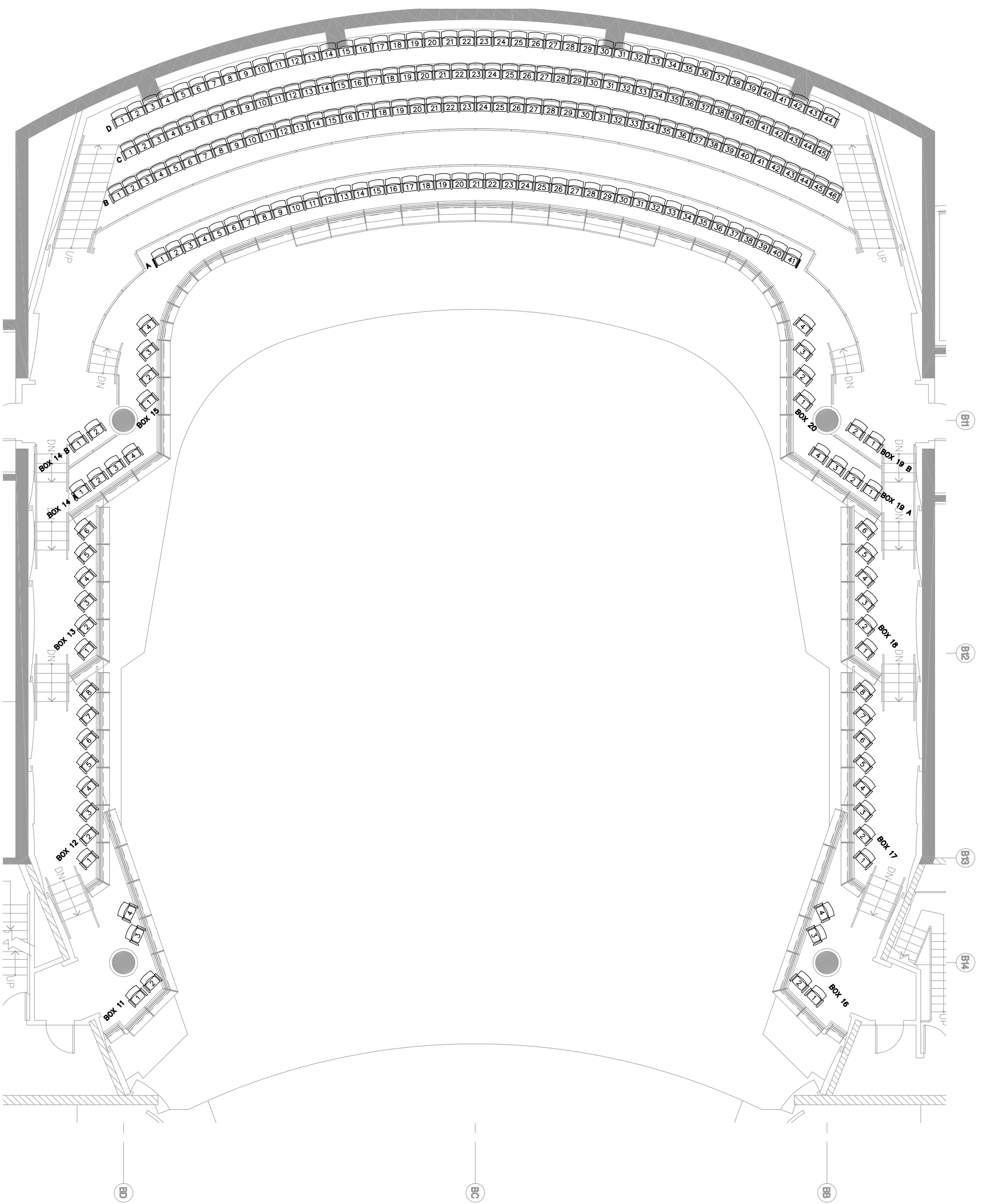
1 PLAN AT BALCONY (SECOND BALCONY) 1/8" = 1'-0"
